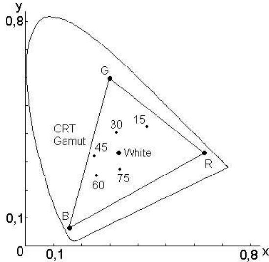
Fig. 3. Color presentation capability of a CRT display containing P22 phosphorus, and the ellipse of the Farnsworth 100 Hue test's color.
