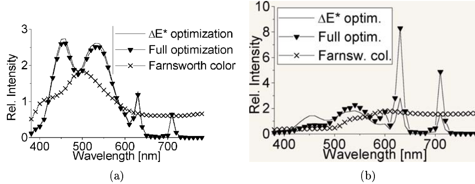
Fig. 4. The reflexive spectrum of Frasnworth cap 15 (a) and cap 45 (b) in comparison with partially and totally optimized (R, G, B)_{DAC} emission.
