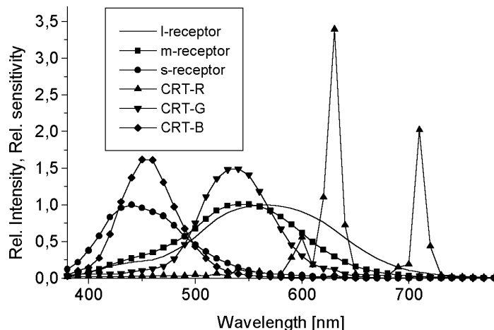
Fig. 1. Emission spectrum of CRT displays containing phosphorus P22 and sensitivity characteristics of the receptors of the human eye.
