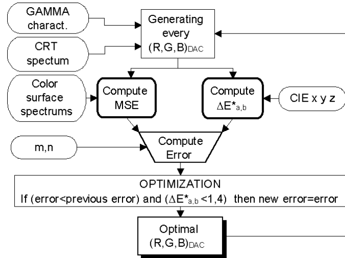
Fig. 2. Algorithm of the optimization procedure.
